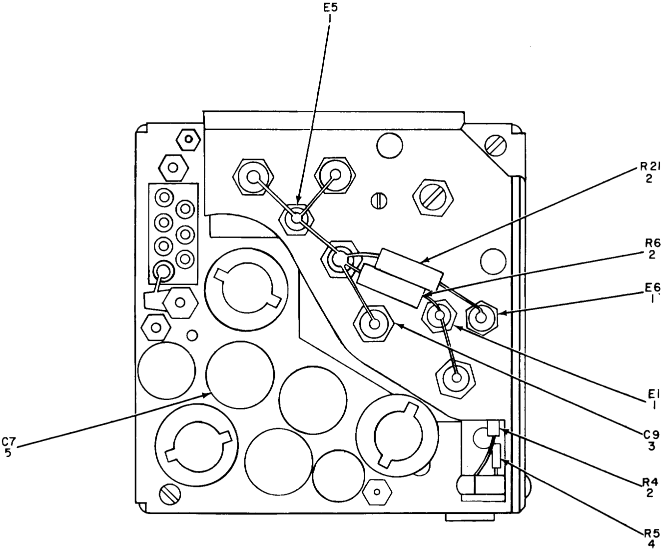
TOP VIEW
