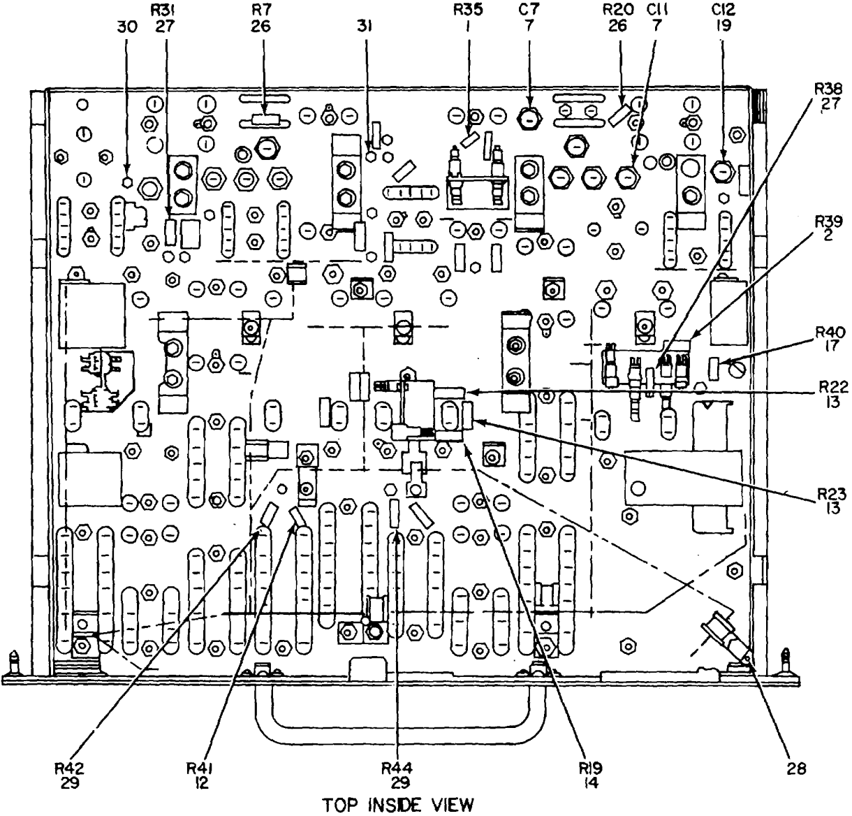
Figure 5. Amplifier-Pilot Regulator AM-708/TCC-8, Repeater Panel, Top and Bottom Views (Sheet 3 of 3).
