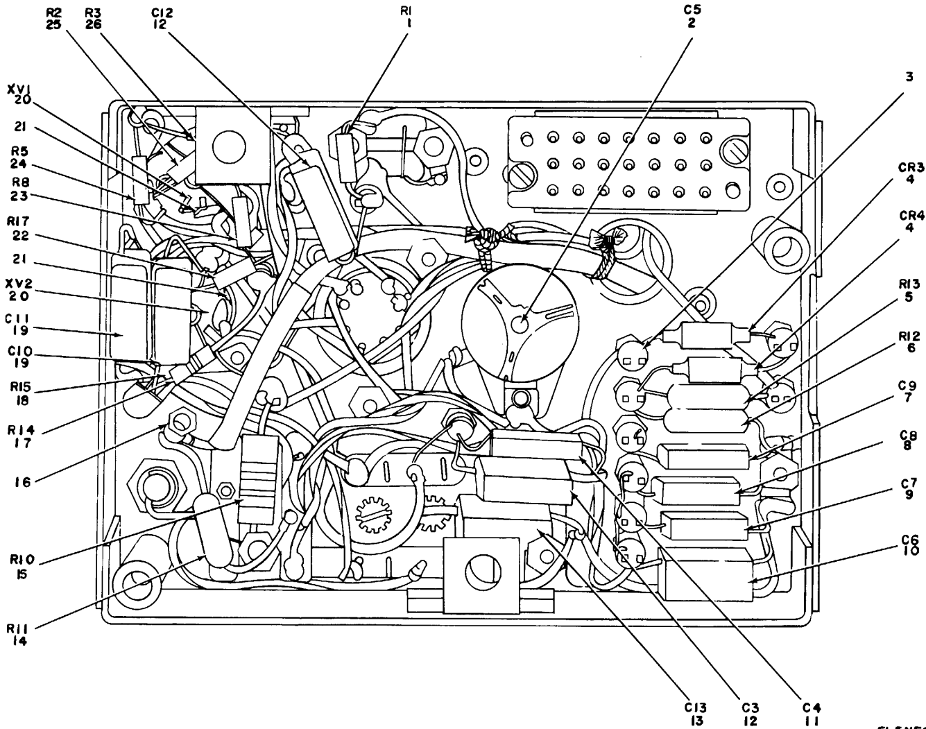
FIGURE 20. RINGER-OSCILLATOR Y101, BOTTOM VIEW.
