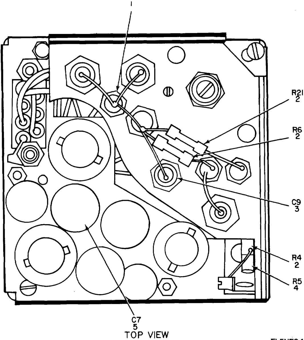
Figure 30. Amplifier, Flat AR2 (Sheet 1 of 2).
