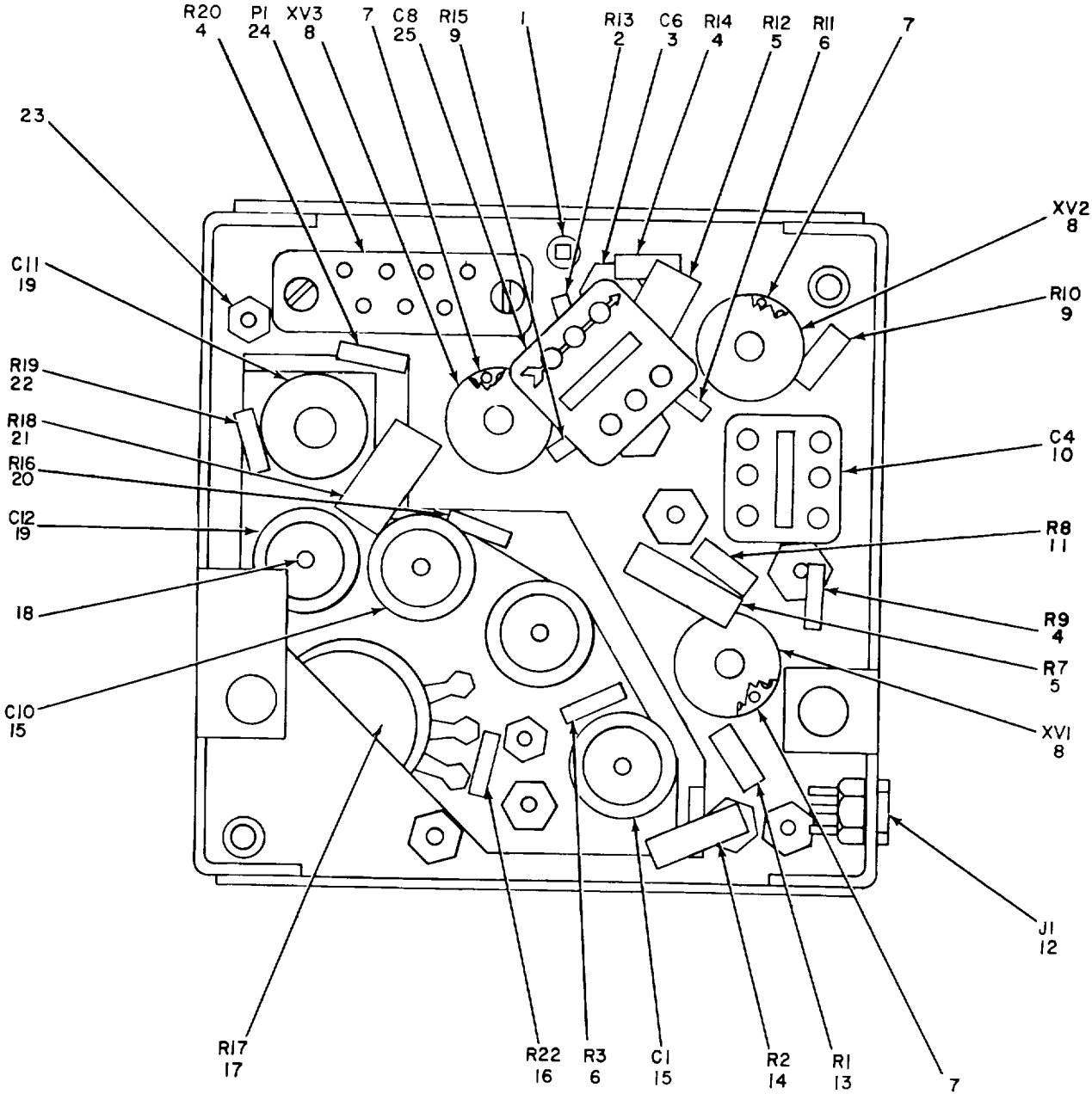
Figure 31. Amplifier, Flat AR2, Bottom View.
