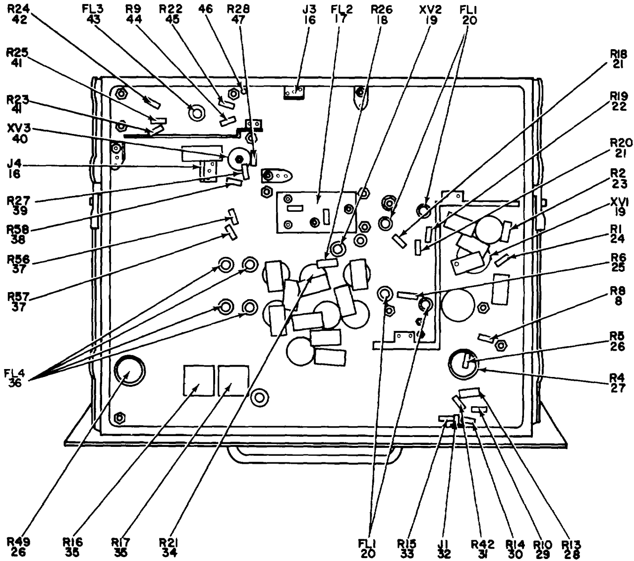
BOTTOM VIEW
