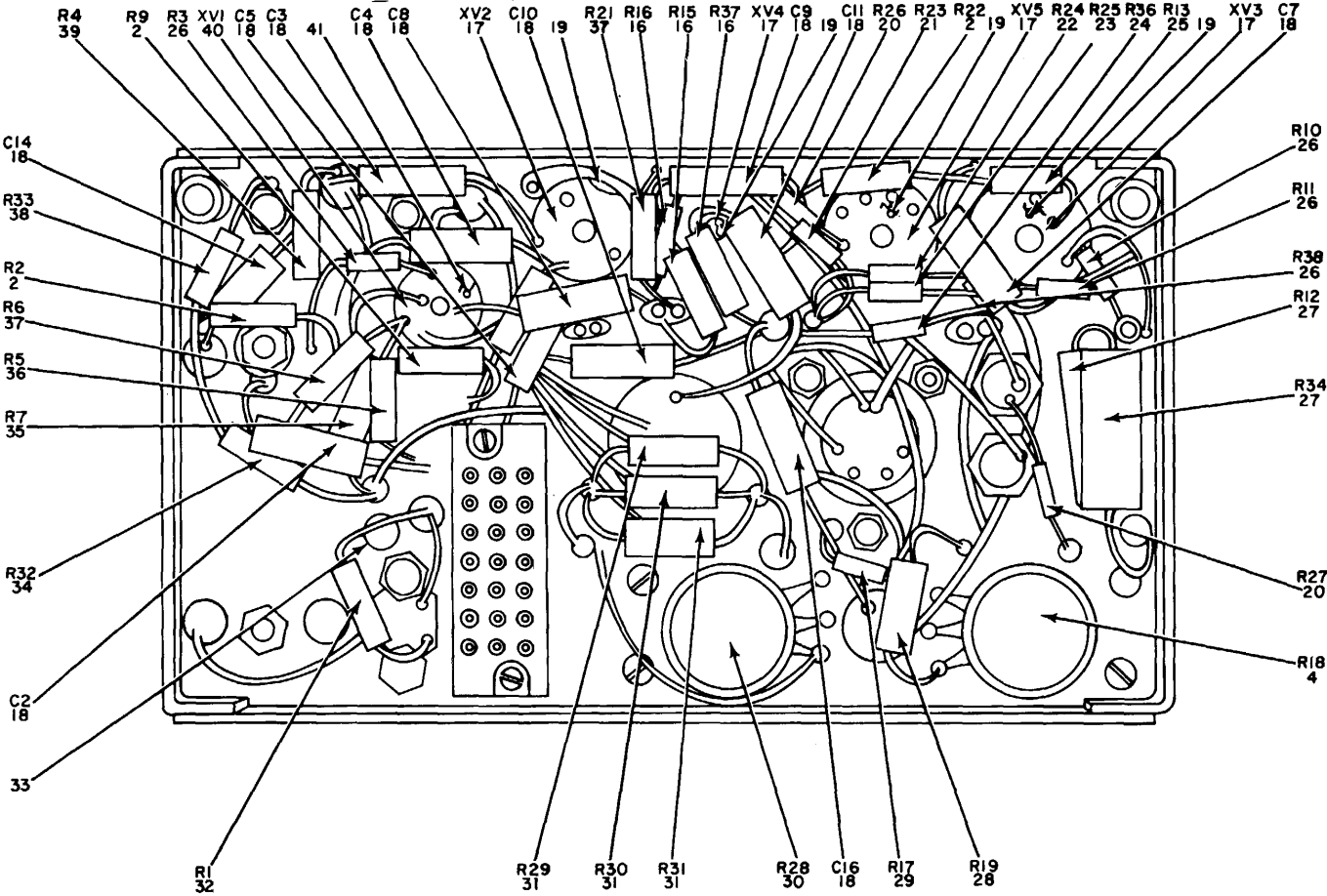
BOTTOM VIEW
