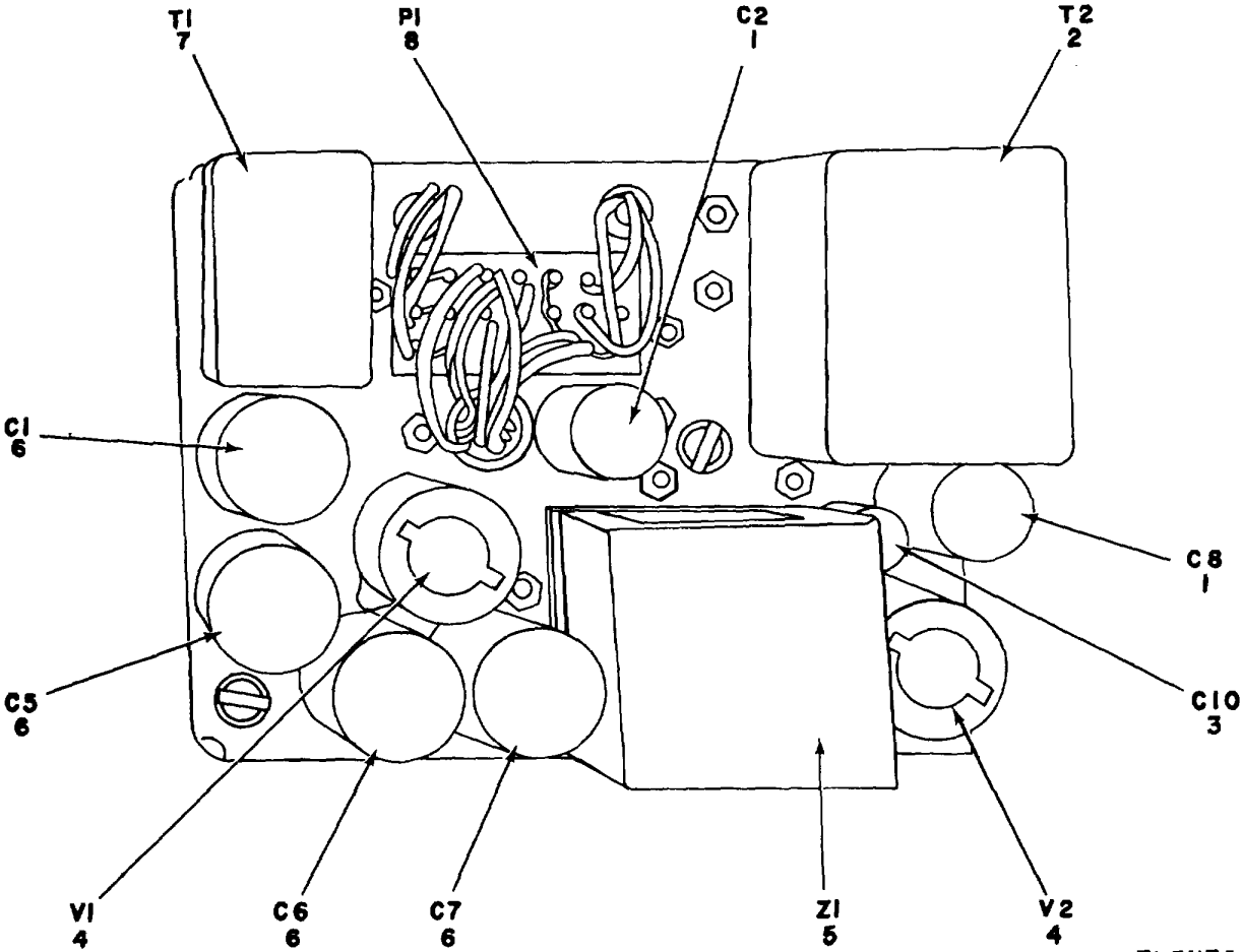
Figure 7. Amplifier, AR-1, AR-2, AR-3, AR-4.
