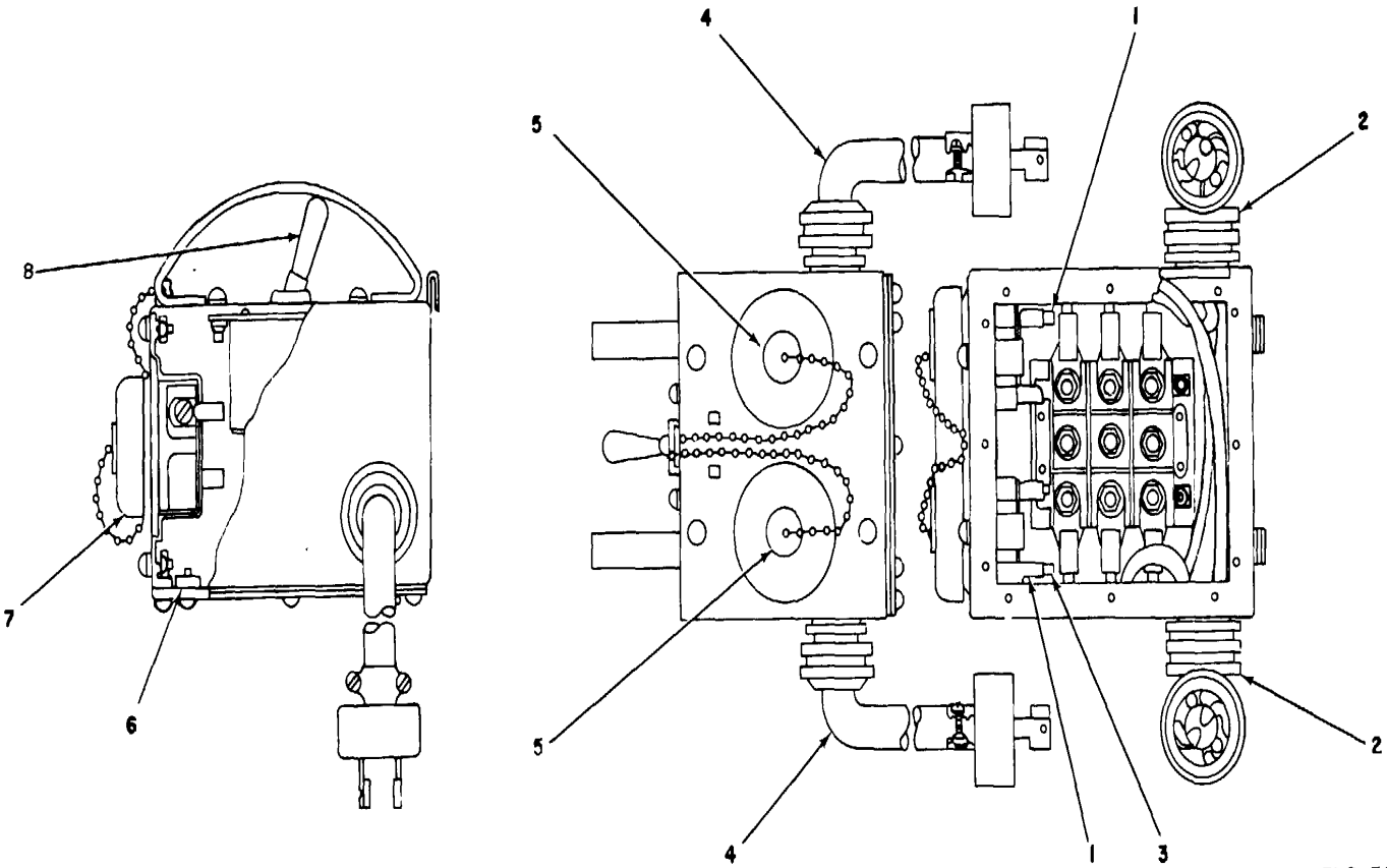
Figure 33. Junction Box J-85/G
