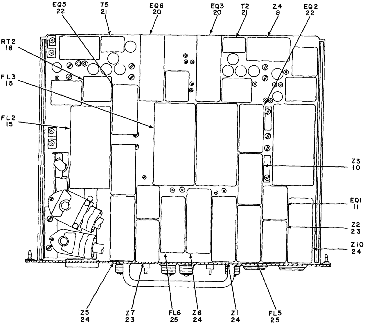
BOTTOM VIEW
