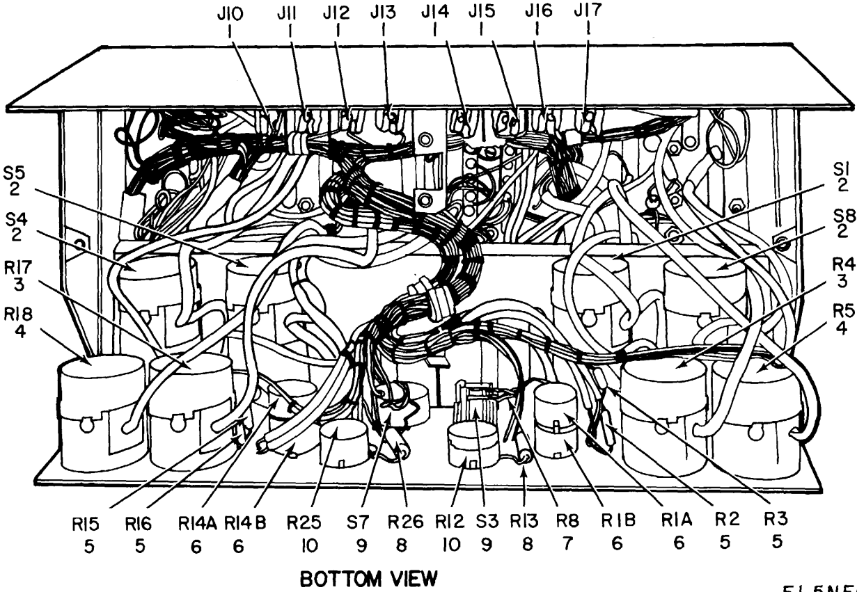
Figure 4. Amplifier-Pilot Regulator AM-708/TCC-8, Repeater Panel (Sheet 1 of 2).
