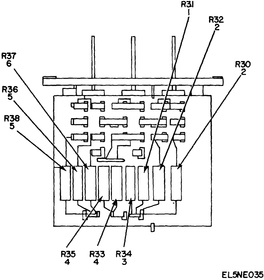
Figure 26. Telephone Test Set TS-761/TCC-8, Switch Assembly, S5.
