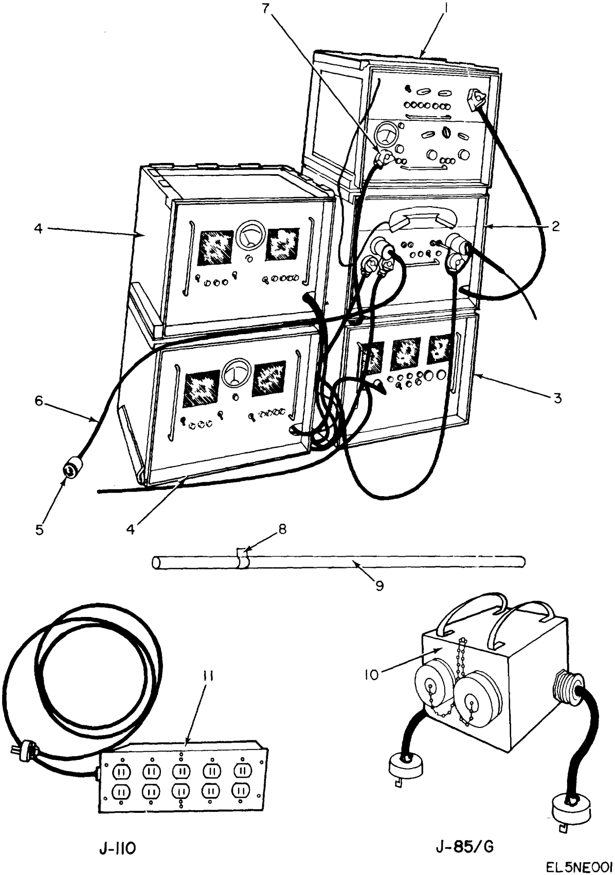
Figure 1. Telephone Repeater AN/TCC-8 and AN/TCC-21.
